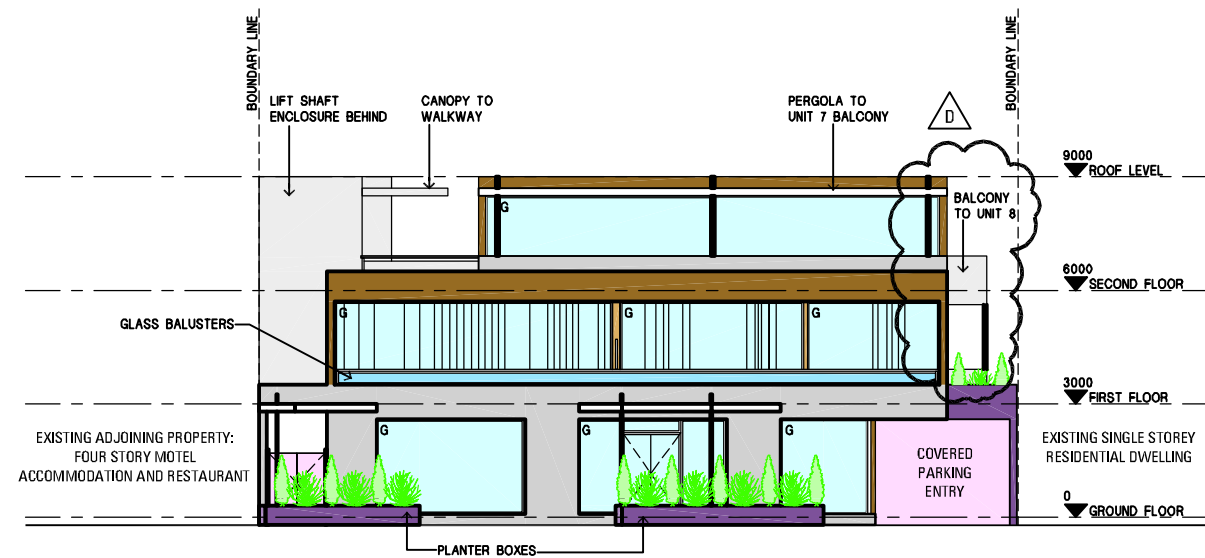
SOUTH ELEVATION- FRONT FACADE SCALE 1:200
